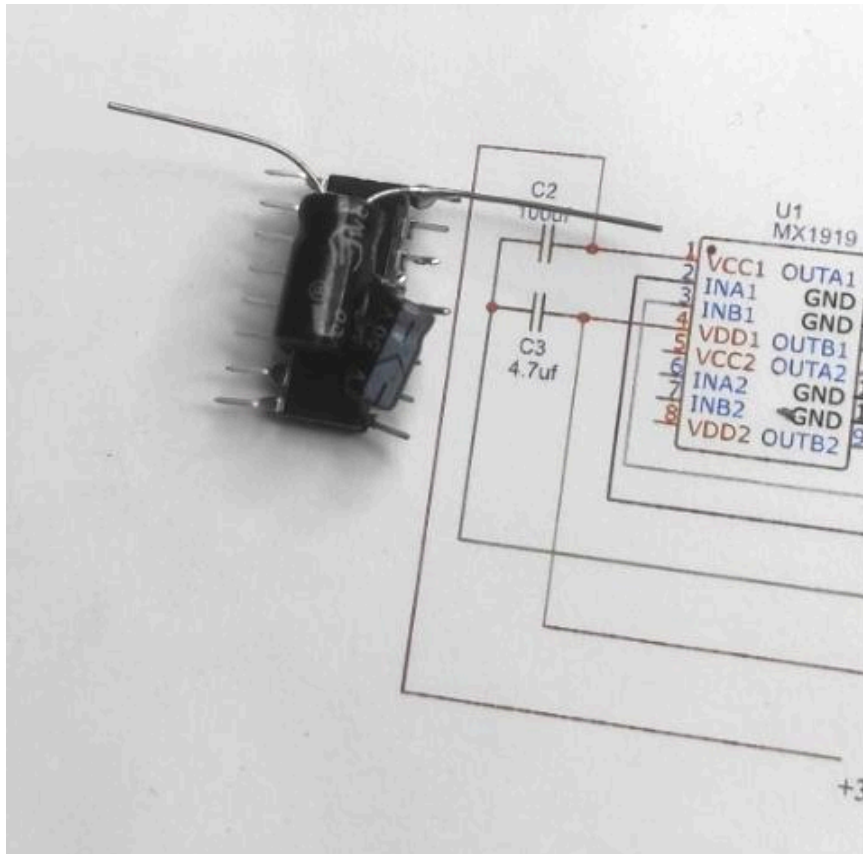
Picture 23: Motor driver assembled according to schematic
