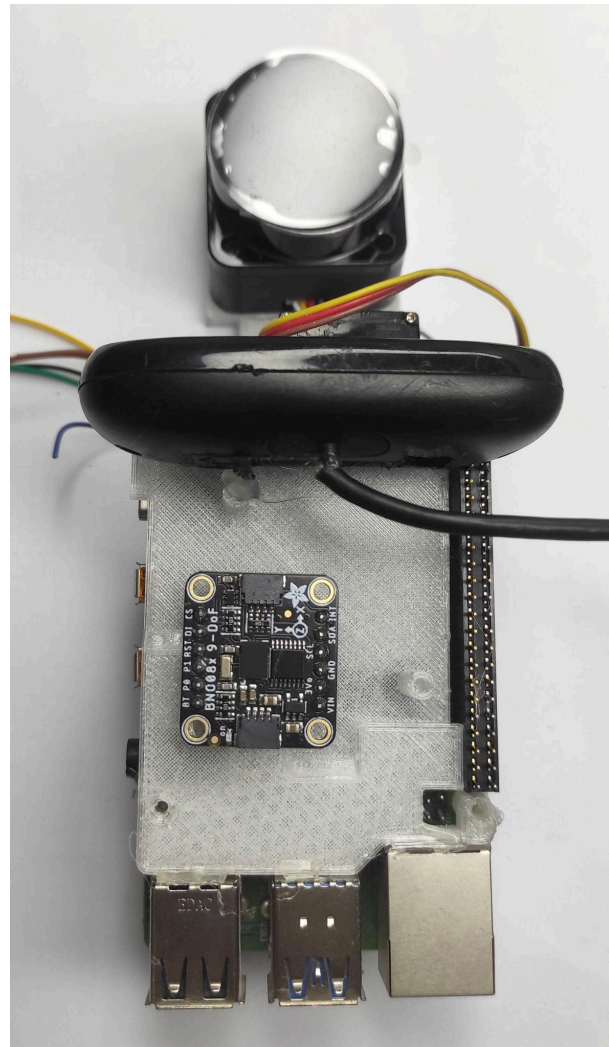
Picture 30: Gyroscope and camera fitted
